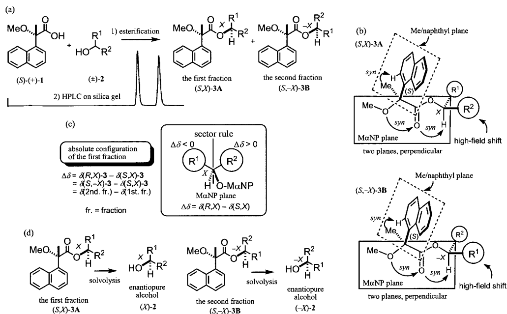
Figure 1. General scheme of enantioresolution and determination of the absolute configuration of the first eluted diastereomeric ester with chiral MaNP acid (S)-(+)-1.
