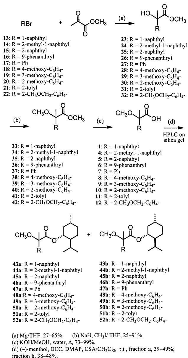
Scheme 1. Preparation of diastereomeric esters from ( - )-menthol and racemic carboxylic acids. The preparation of MaNP acid esters 43a/43b and M9PP acid esters 46a/46b has been reported. [12,19]
