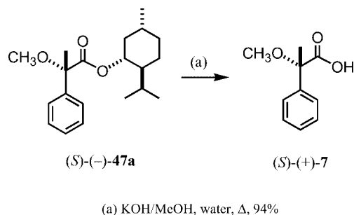
Scheme 2. Recovery of enantiopure carboxylic acid (S)-(+)- 7 .
