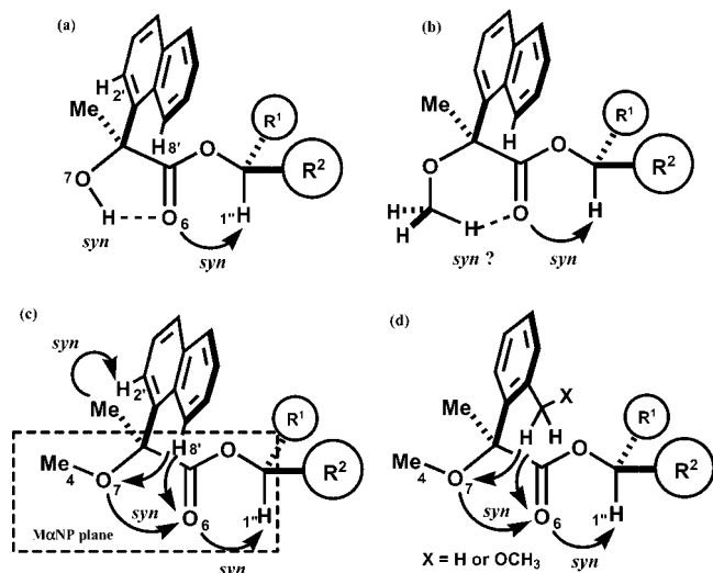
Figure 5. The possible conformers of MaNP and related acid esters stabilizing the syn-syn conformation.
