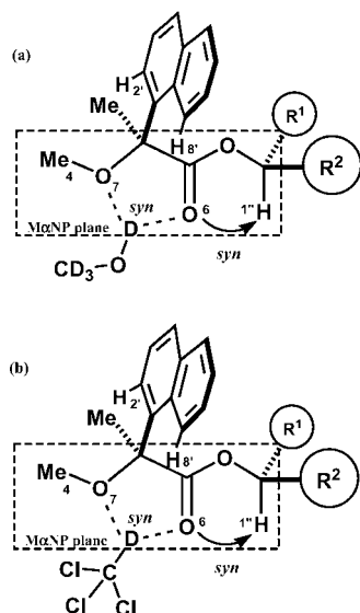
Figure 6. The possible syn-syn conformation of MaNP esters stabilized by solvation: hydrogen bonding or hydrogen-bonding-like interaction.
