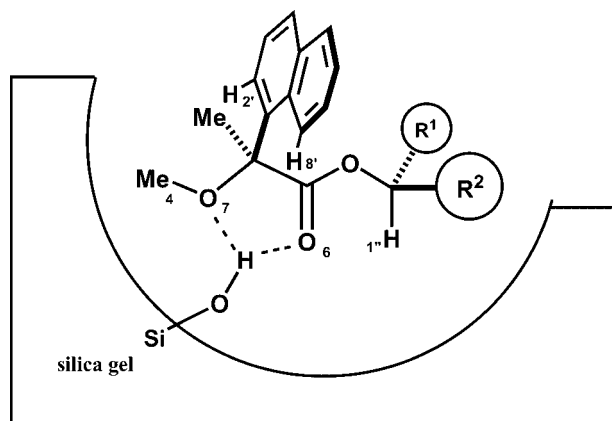
Figure 7. The plausible mechanism of the diastereomeric discrimination of MaNP esters in the holes of silica gel, where ester molecules are adsorbed by hydrogen bonding.
