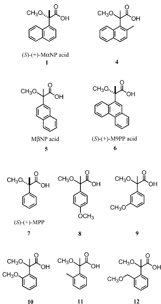
Figure 2. MaNP acid ( S )-(+)- 1 and related acids.
