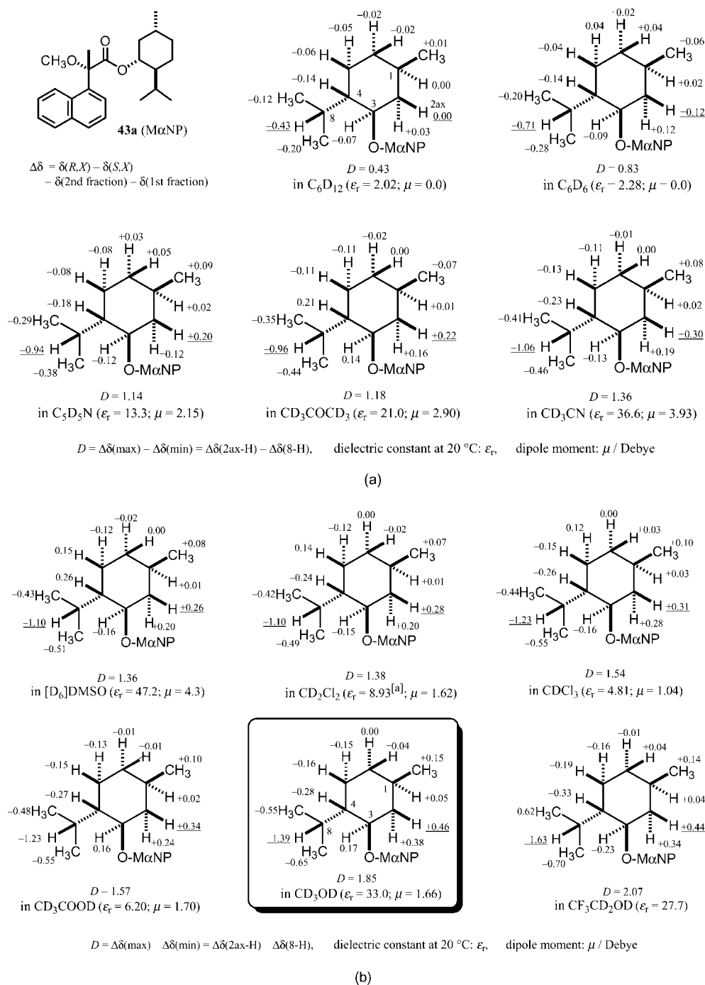
Figure 4. (a) Solvent effect on the ^1\text{H} NMR anisotropy data of (1 R ,3 R ,4 S )-menthol MαNP acid esters 43a and 43b . \Delta\delta [= \delta(2\text{nd fraction}) - \delta(1\text{st fraction}) ] and D values are given in ppm. Spectra were recorded at 600 MHz. (b) Solvent effect on the ^1\text{H} NMR anisotropy data of (1 R ,3 R ,4 S )-menthol MαNP acid esters 43a and 43b . \Delta\delta [= \delta(2\text{nd fraction}) - \delta(1\text{st fraction}) ] and D values are given in ppm. Spectra were recorded at 600 MHz. [a] Dielectric constant at 25 °C. The \Delta\delta values in [\text{D}]\text{chloroform} were taken from ref. [12]
