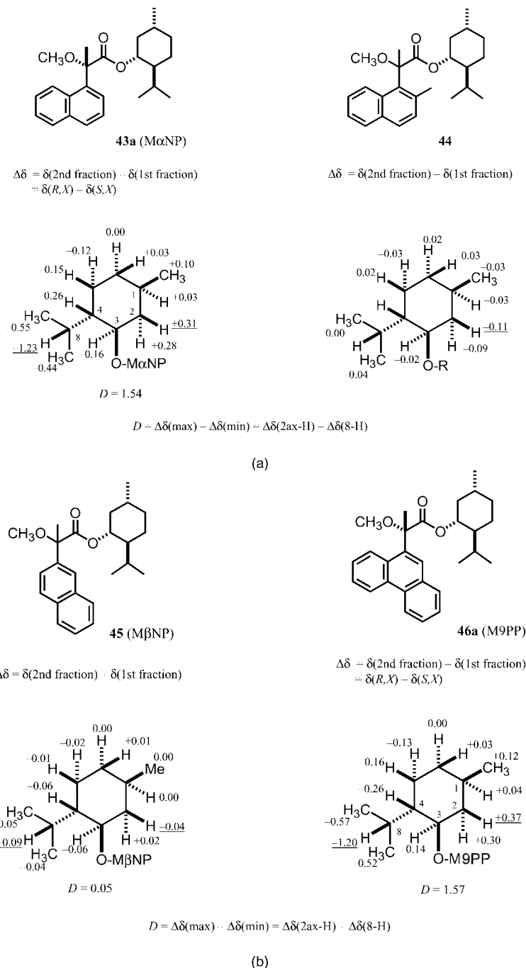
Figure 3. (a) ^1\text{H} NMR anisotropy effects of (1 R ,3 R ,4 S )-menthol \text{MaNP} acid esters 43a (first eluted fraction), 43b (second eluted fraction), and related acid esters 44 . \Delta\delta \{= \delta(\text{2nd fraction}) - \delta(\text{1st fraction})\} and D values are shown in ppm. Spectra were recorded at 600 MHz in \text{CDCl}_3 . For esters 44 , the D value was not calculated because of overlap of proton signals. The \Delta\delta values of esters 43a/43b were taken from ref. [12] (b) ^1\text{H} NMR anisotropy effects of (1 R ,3 R ,4 S )-menthol esters 45 and 46 . \Delta\delta \{= \delta(\text{2nd fraction}) - \delta(\text{1st fraction})\} and D values are given in ppm. Spectra were recorded at 600 MHz in \text{CDCl}_3 . The \Delta\delta values of esters 46a/46b were taken from ref. [19] (c) ^1\text{H} NMR anisotropy effects of (1 R ,3 R ,4 S )-menthol esters 47 , 48 , and 49 . \Delta\delta \{= \delta(\text{2nd fraction}) - \delta(\text{1st fraction})\} and D values are given in ppm. Spectra were recorded at 600 MHz in \text{CDCl}_3 . (d) ^1\text{H} NMR anisotropy effects of (1 R ,3 R ,4 S )-menthol esters 50 , 51 , and 52 . \Delta\delta \{= \delta(\text{2nd fraction}) - \delta(\text{1st fraction})\} and D values are given in ppm. Spectra were recorded at 600 MHz in \text{CDCl}_3 .
